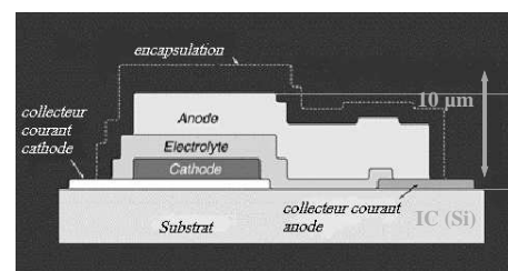
Fig. 17: Micro-battery in "Above IC" technology
