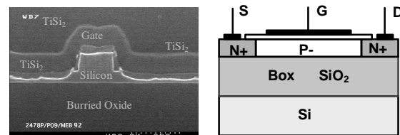
Fig. 3: SOI process and basic transistor
