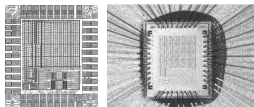
Fig 14: Test chip
