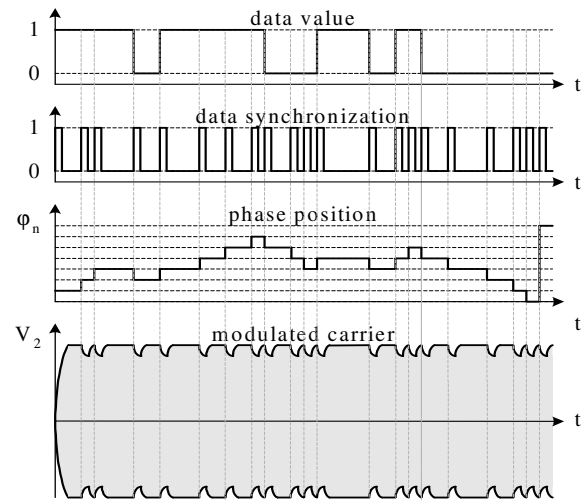
Fig 13: Chronograms
