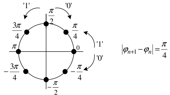
Fig 12: The modulation/coding scheme
