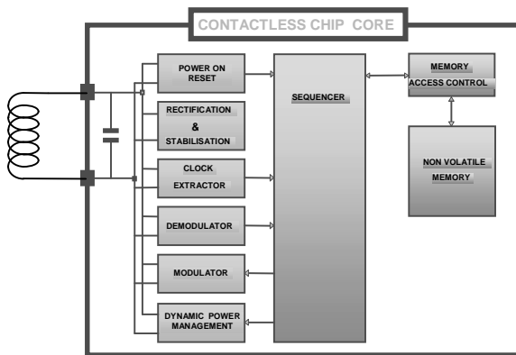
Fig. 1: Basic architecture of RFID chip
