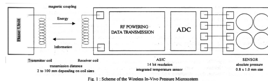
Fig. 1: Scheme of the Wireless In-Vivo Pressure Microsystem
