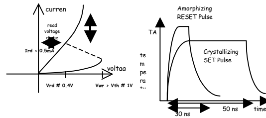
Fig 9: I(V) and bit cells programming curves
