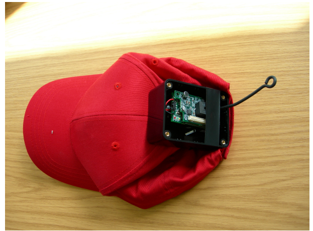
Figure 4: A MICA2 mote [6] with MTS310 sensor board [7] attached to a baseball hat. These are worn by players of Trove, during the game.
