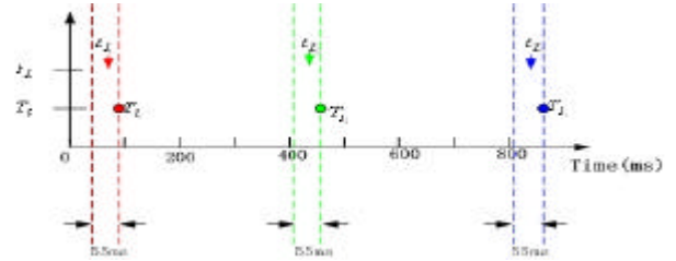
Figure 5: Timing relation between t_{Lx} and T_{Lx} ( x=1,2,\dots ).
