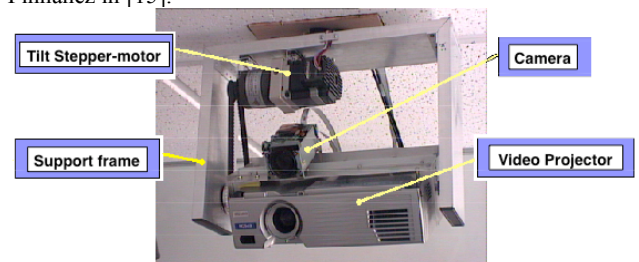
Figure 5. The Steerable Camera-Projector (SCP) pair.
