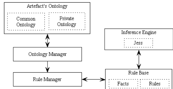
Figure 3: System's architecture.
